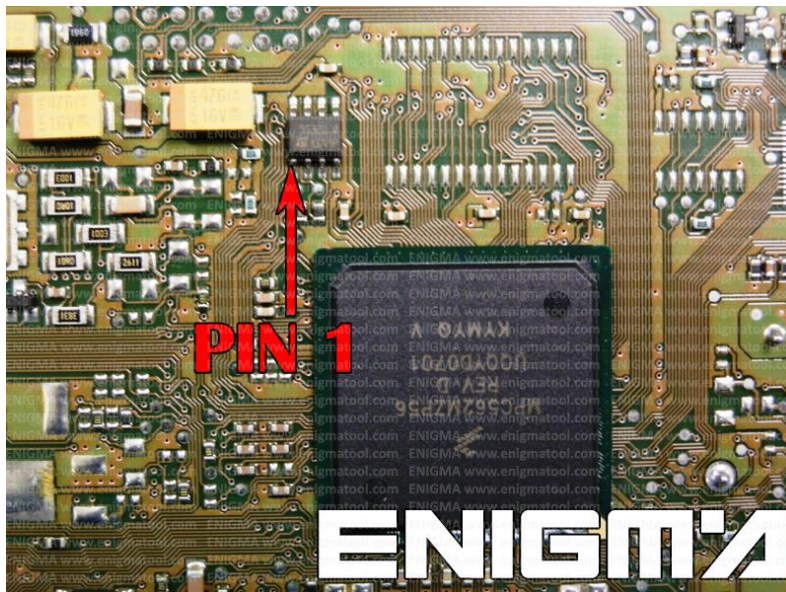
PHOTO 1: Connect cable C4 to EEPROM memory according to the picture above.
